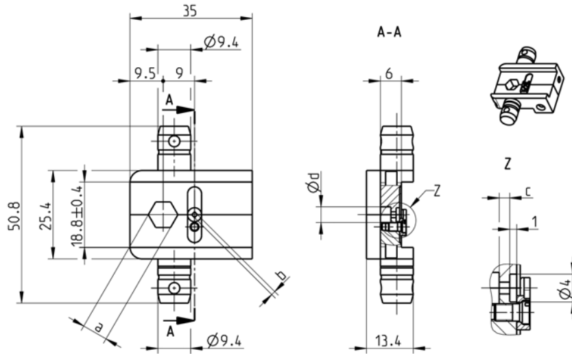
Simplified view without mounting steel sheet and screw.
