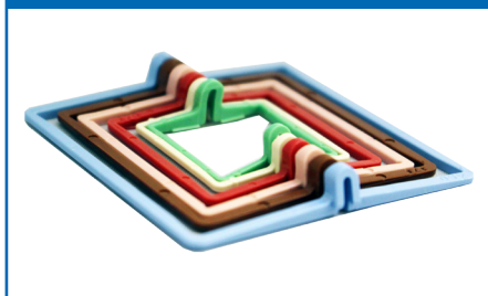
superGRIP™ Frame (above) & Spring Clips (below)
